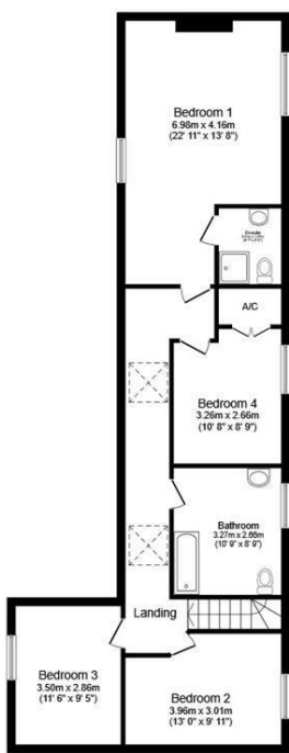
First Floor Floor area 89.6 sq.m. (964 sq.ft.)
